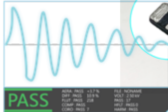
LAPLACIAN Comparison
