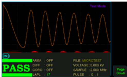
LAPLACIAN Comparison
